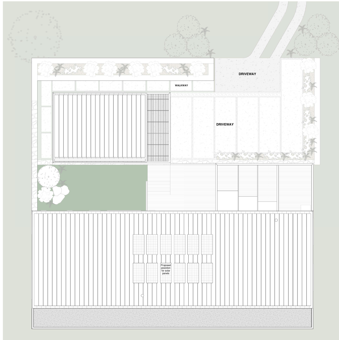
2-BED UNIT ROOF PLAN
