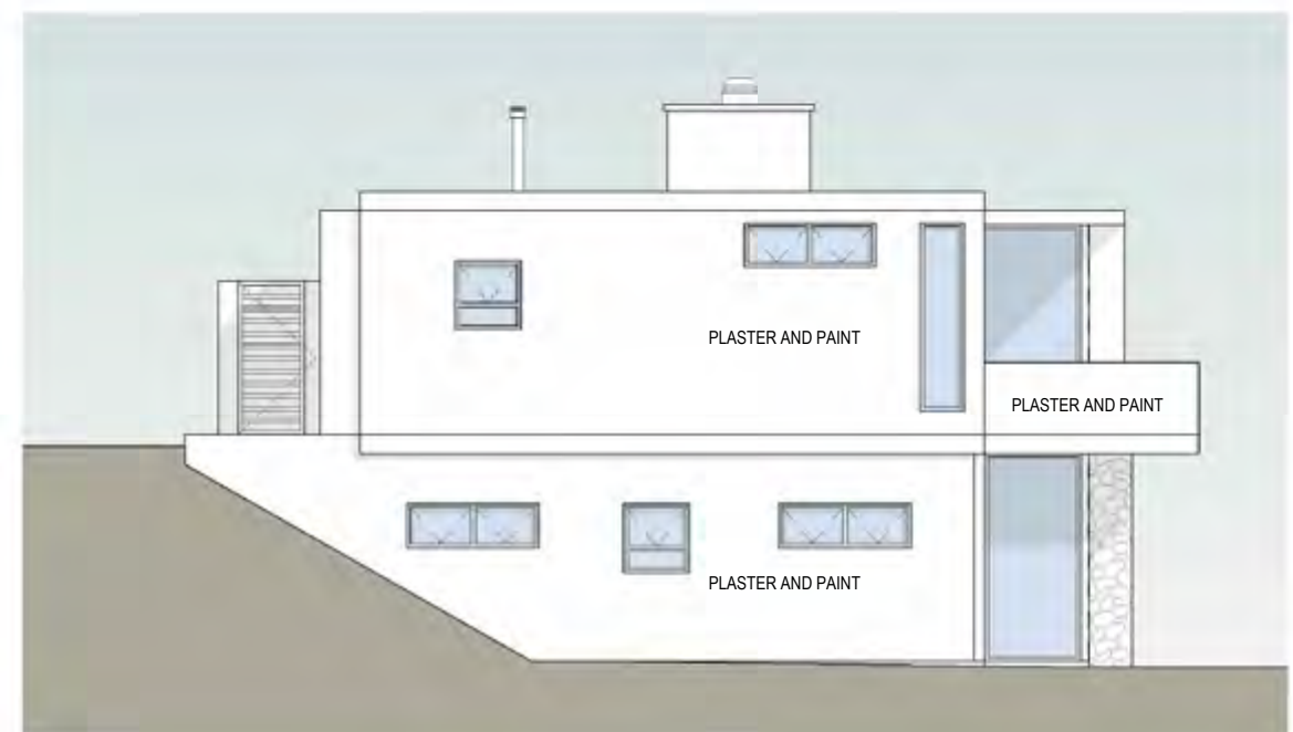
ELEVATION WEST
