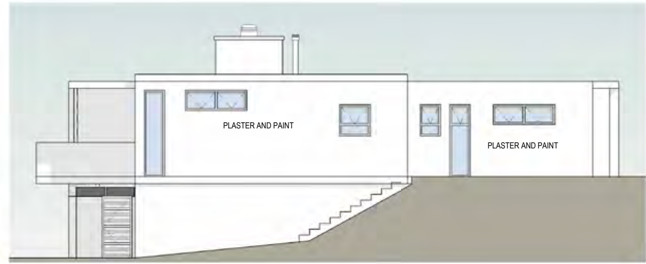
ELEVATION EAST
