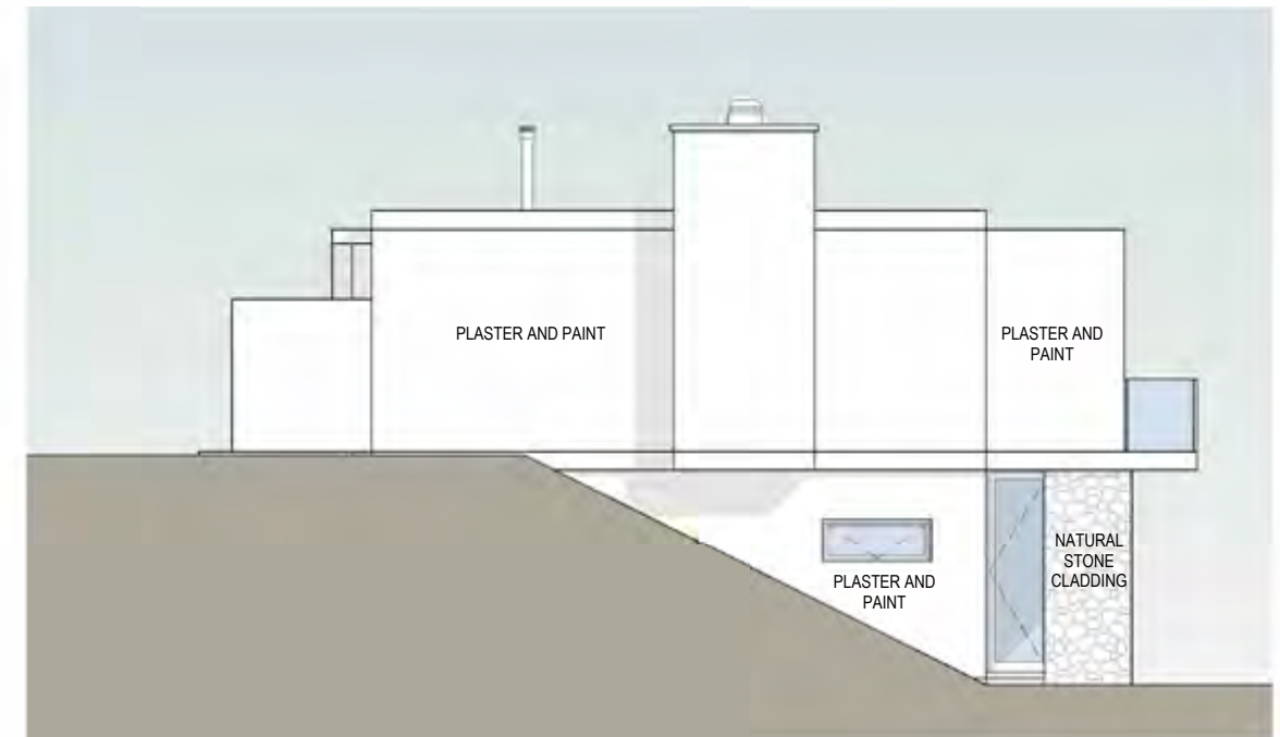
ELEVATION WEST
