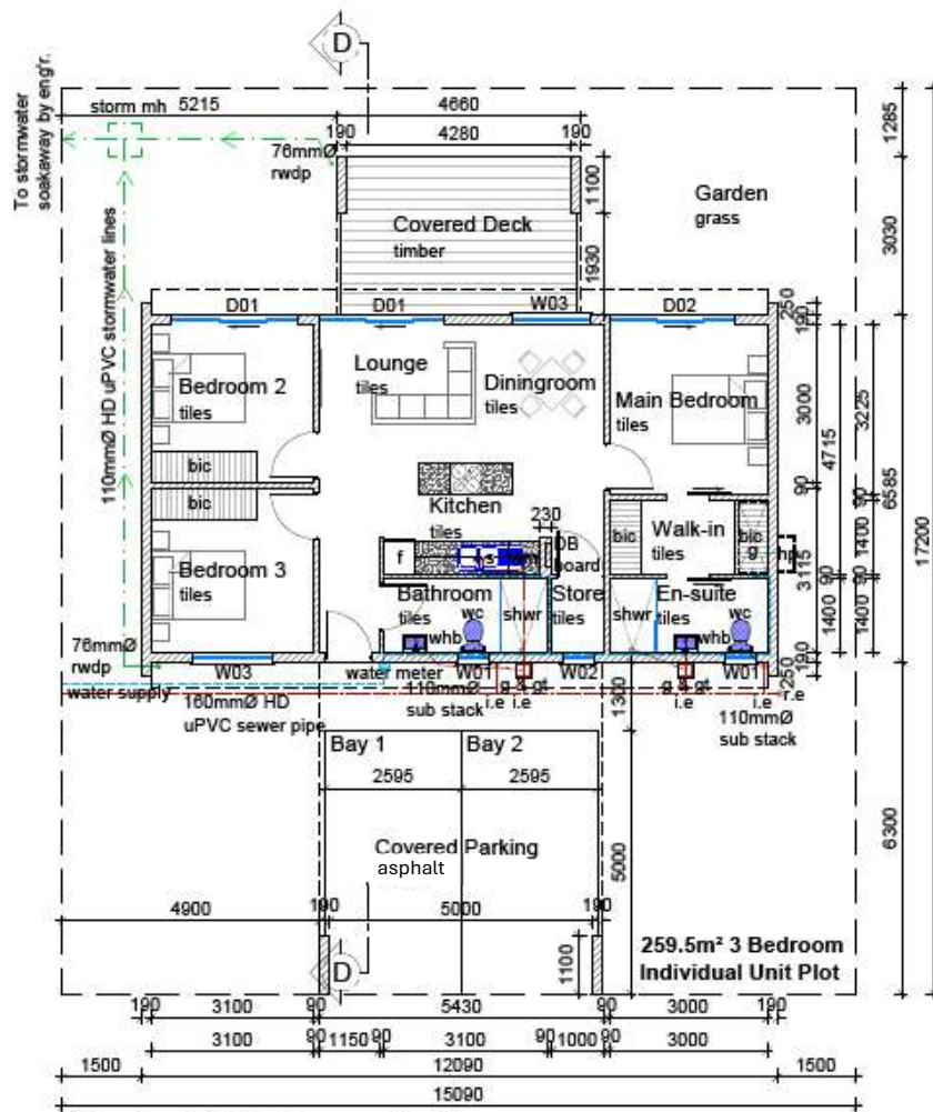
Typical 3 Bedroom Unit
