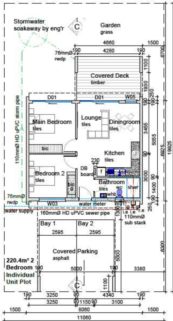
Typical 2 Bedroom Unit
