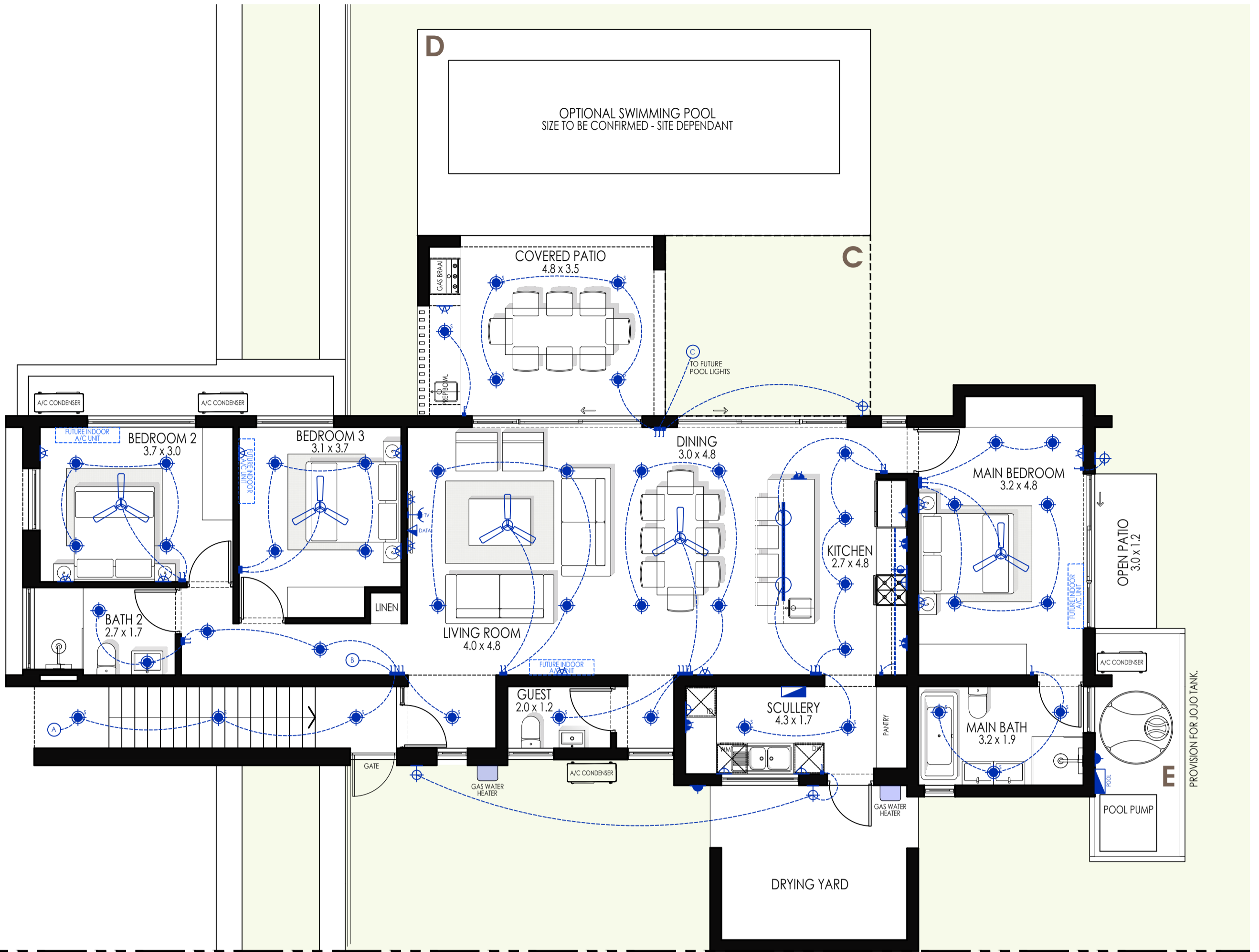
UPPER LEVEL PLAN
