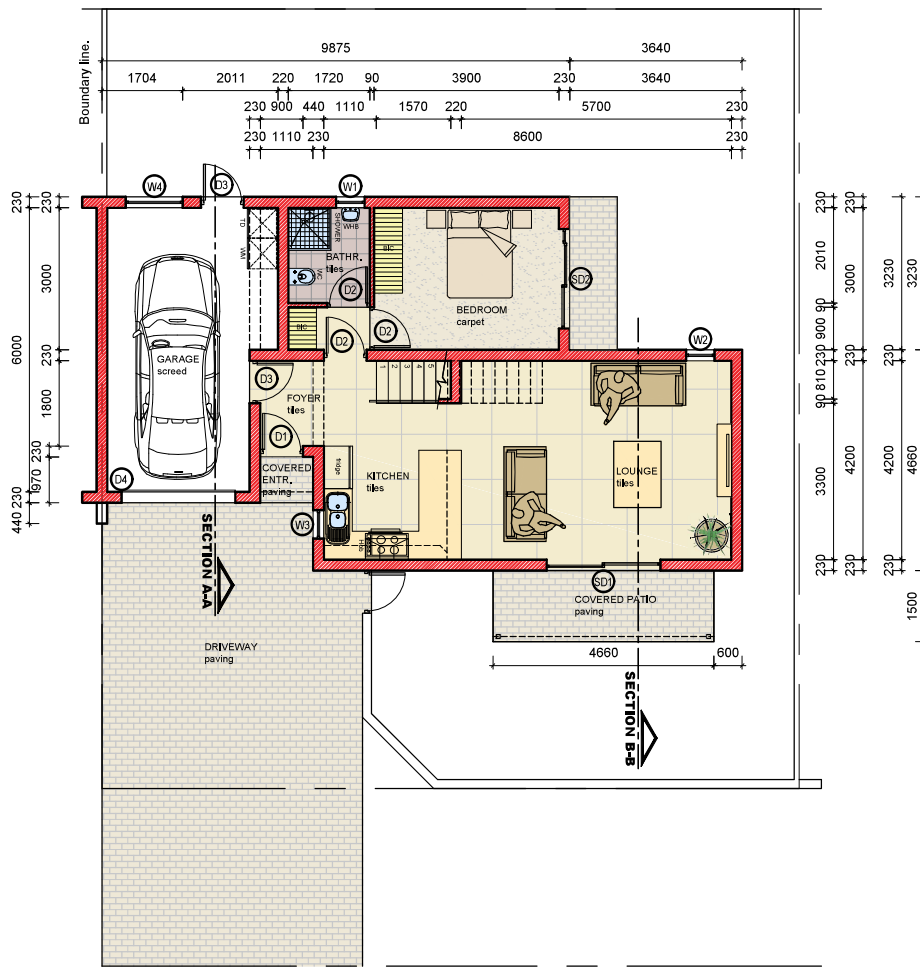
SITE AND GROUND FLOOR PLAN SCALE 1:100
