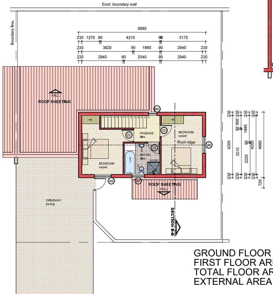
SITE AND FIRST FLOOR PLAN SCALE 1:100
