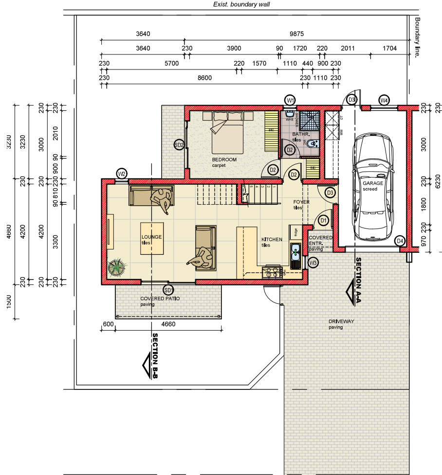
SITE AND GROUND FLOOR PLAN SCALE 1:100
