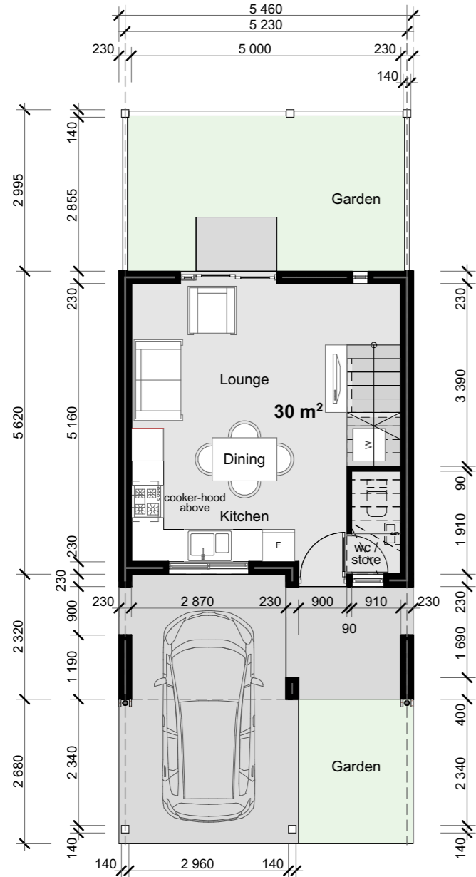
2 BEDROOM UNIT GF PLAN TYPE - B
