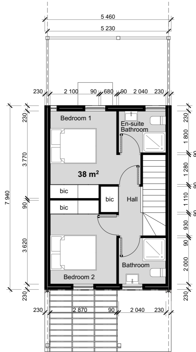
2 BEDROOM UNIT 1st FLOOR PLAN TYPE - B
