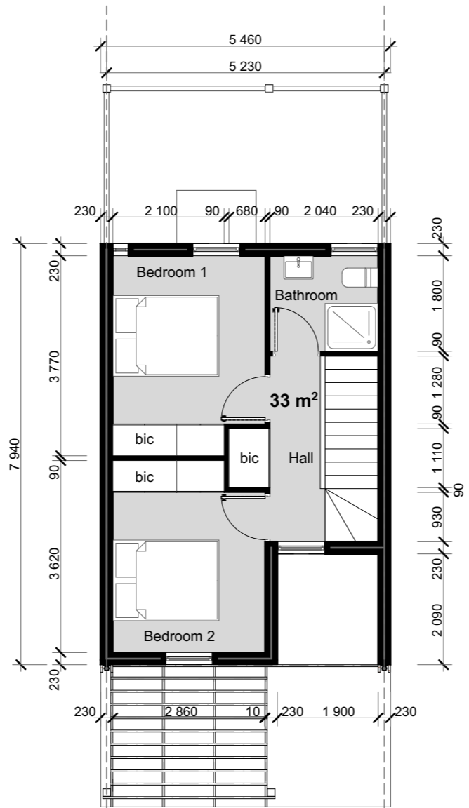
2 BEDROOM UNIT 1st FLOOR PLAN TYPE - A
