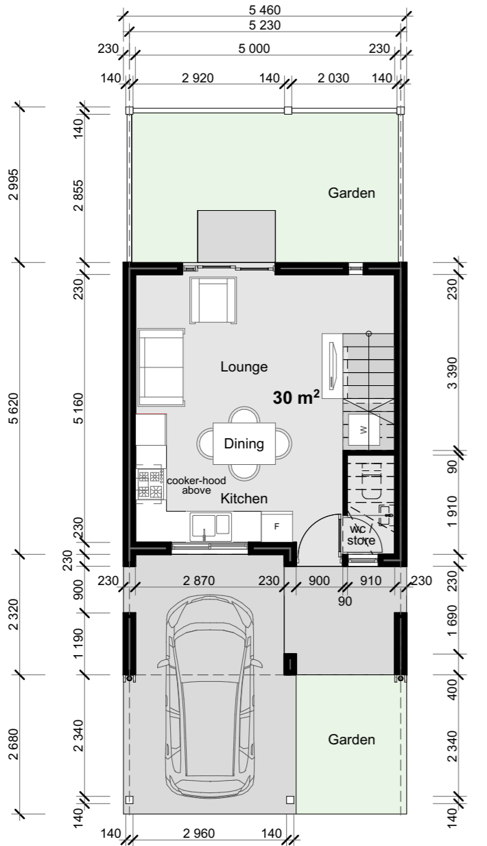
2 BEDROOM UNIT GF PLAN TYPE - A
