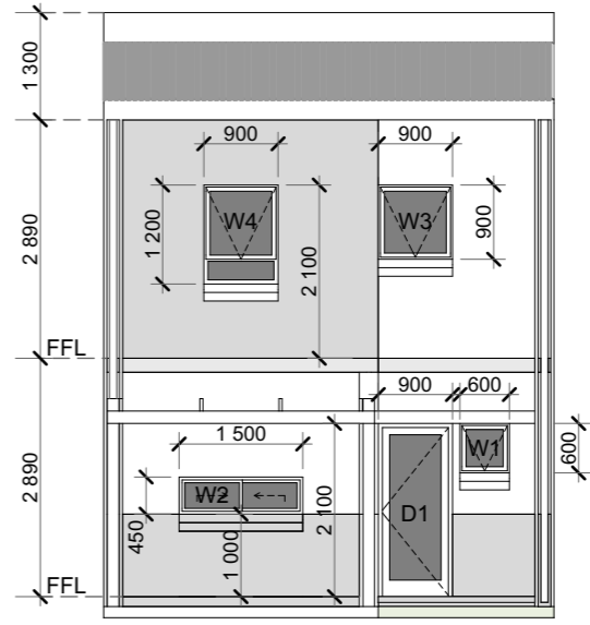
STREET VIEW 1:100
