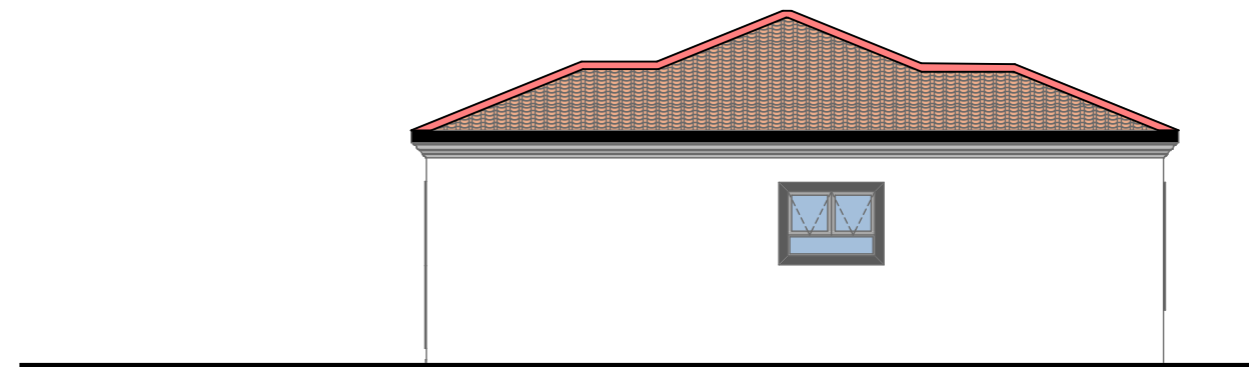
SIDE ELEVATION 1
