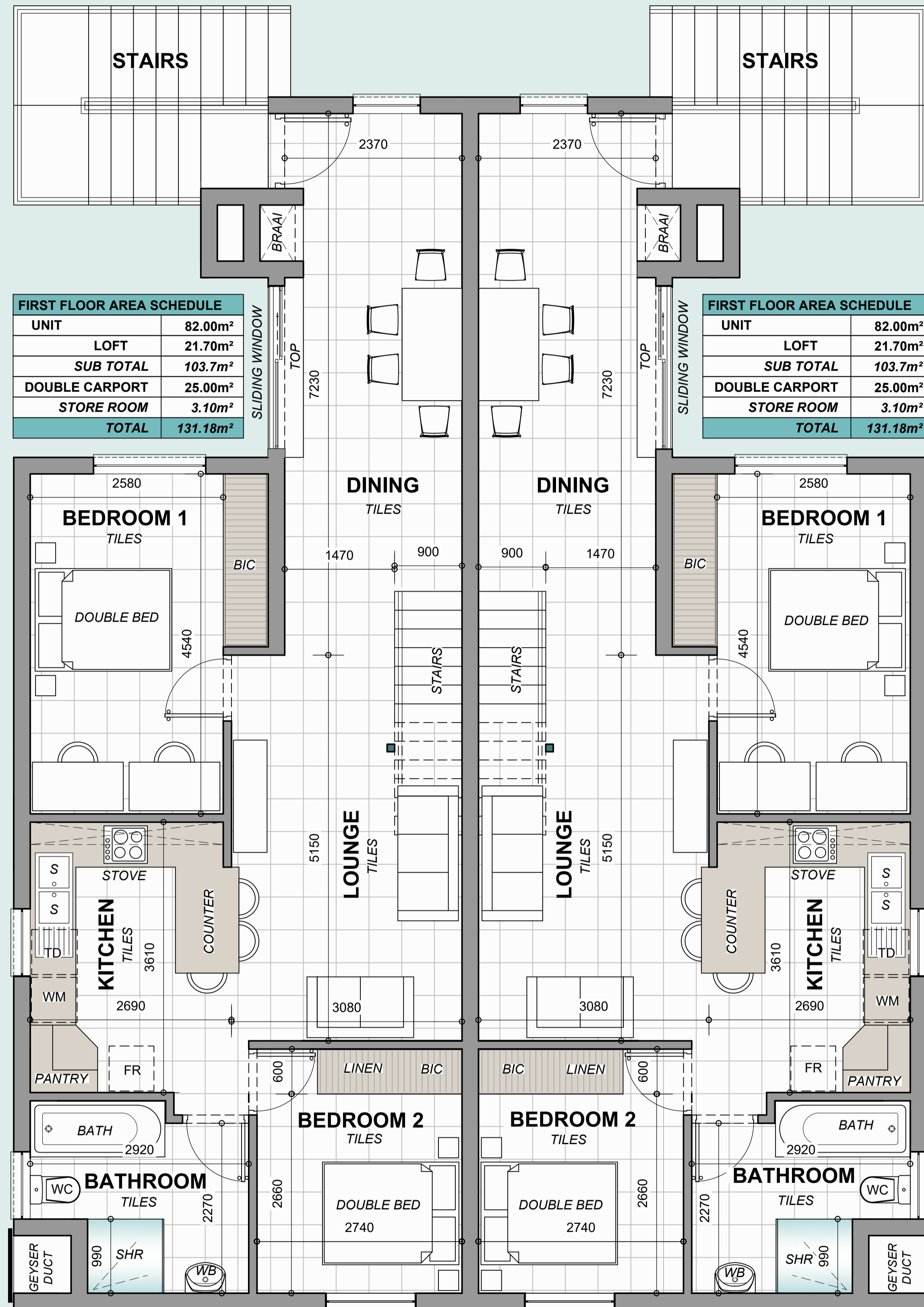
FIRST FLOOR PLAN NOT TO SCALE
