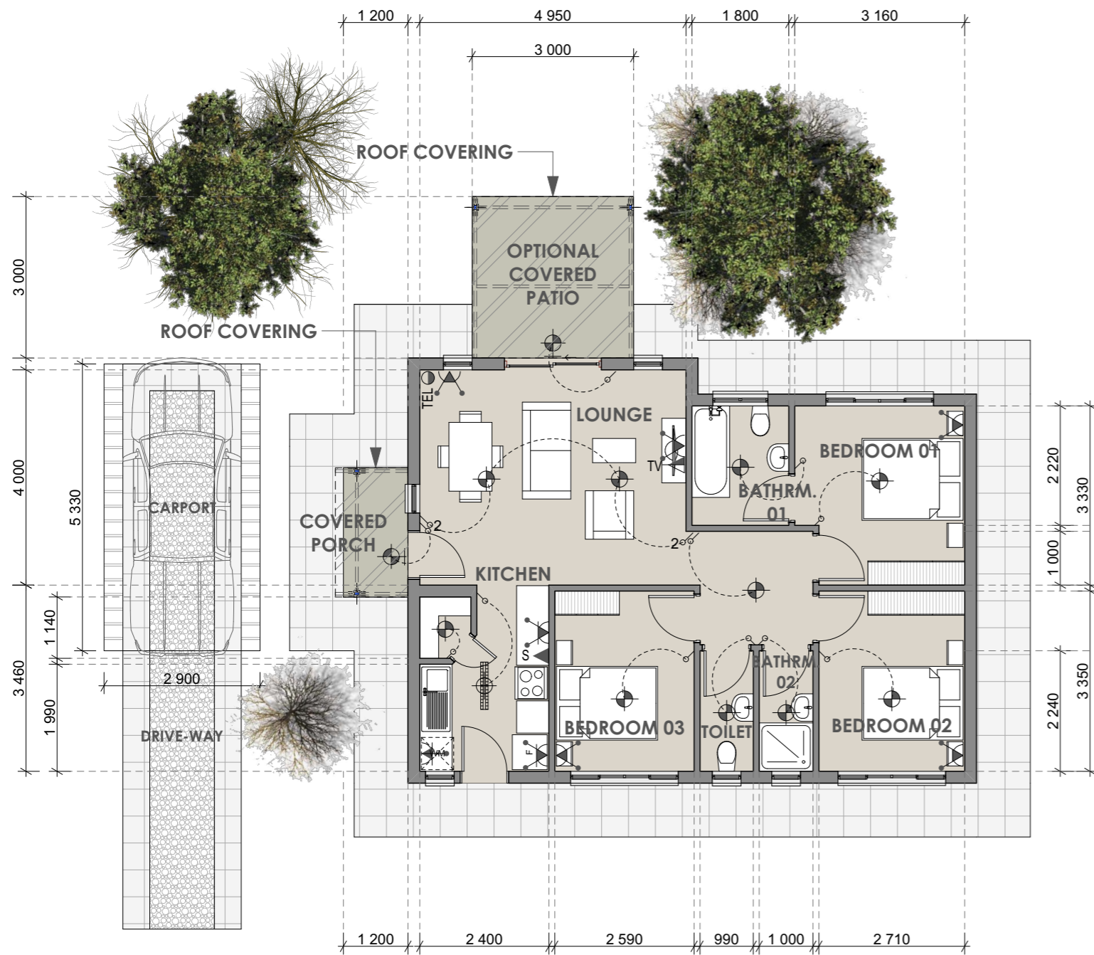
GROUND STOREY PLAN Scale 1:100
