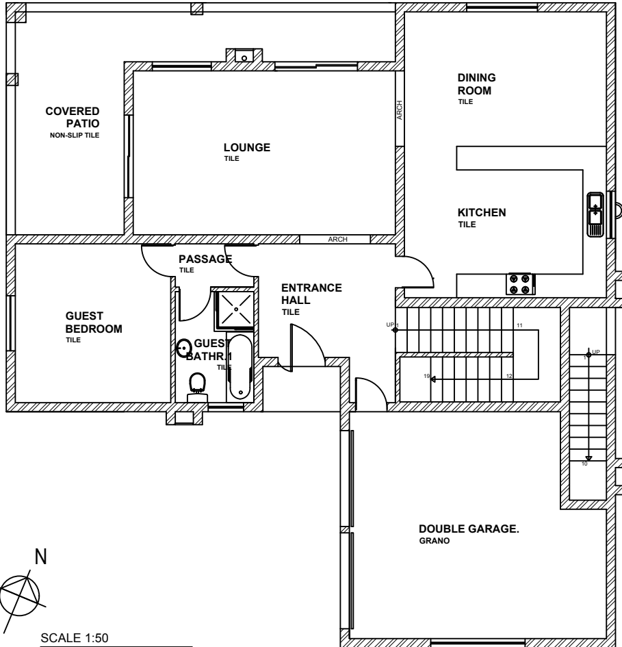
SCALE 1:50 GROUND FLOOR PLAN
