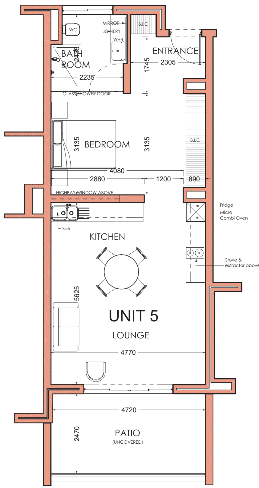
UNIT LAYOUT PLAN
