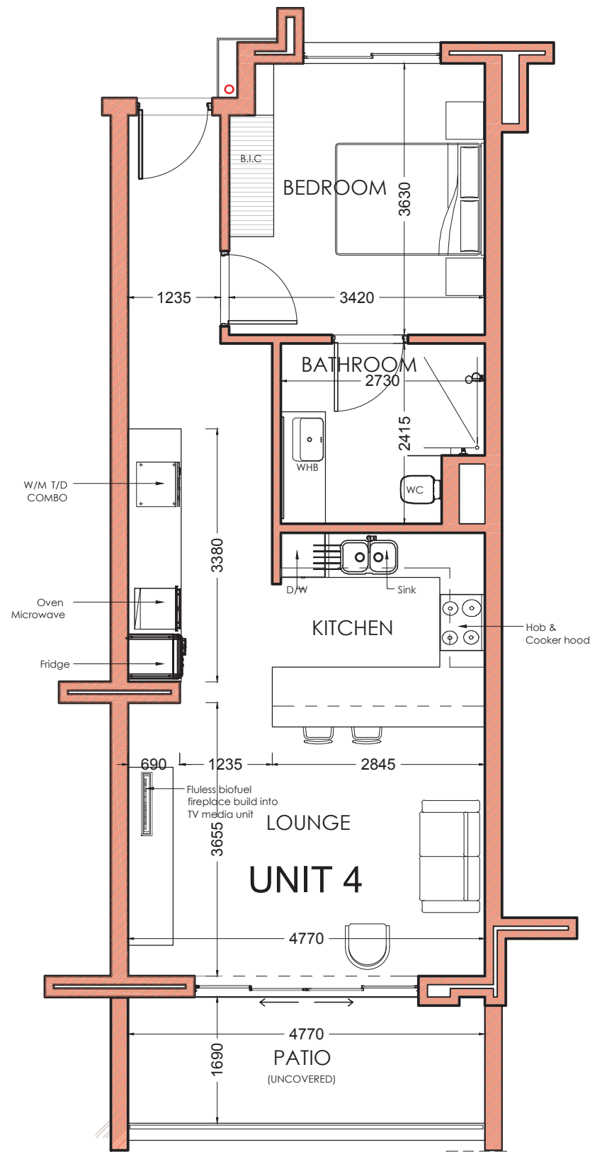
UNIT LAYOUT PLAN
