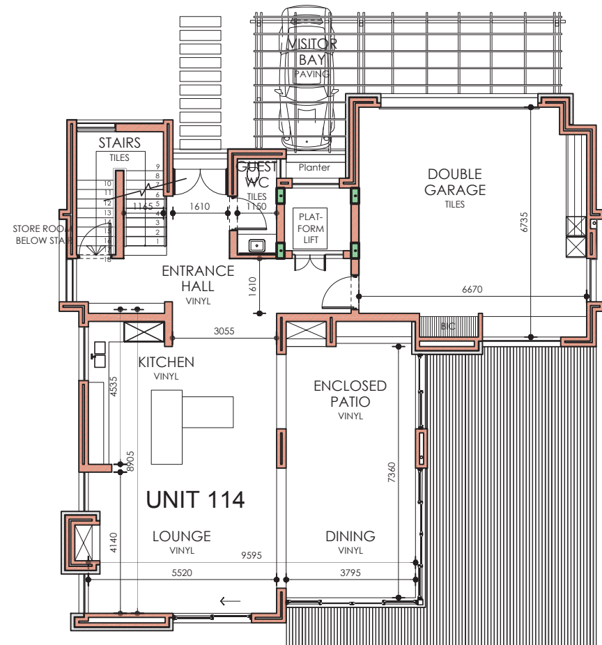
GROUND FLOOR UNIT LAYOUT PLAN
