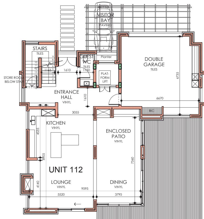
GROUND FLOOR UNIT LAYOUT PLAN
