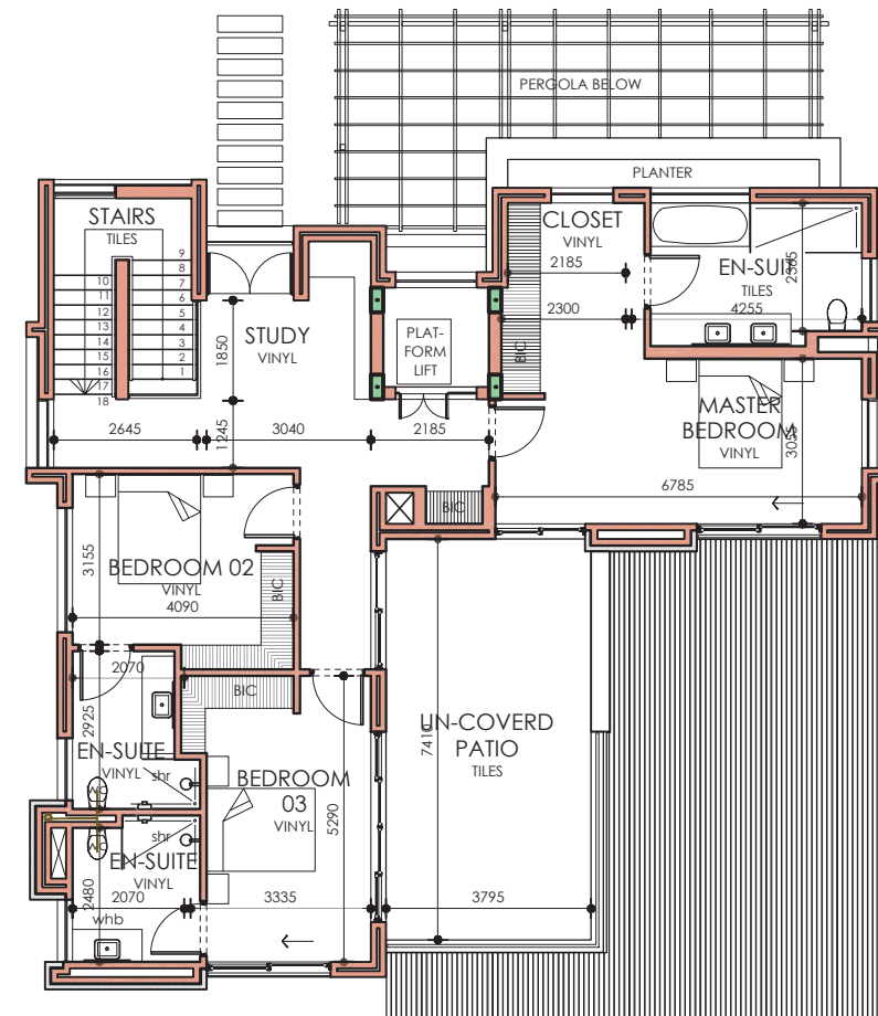
FIRST FLOOR UNIT LAYOUT PLAN
