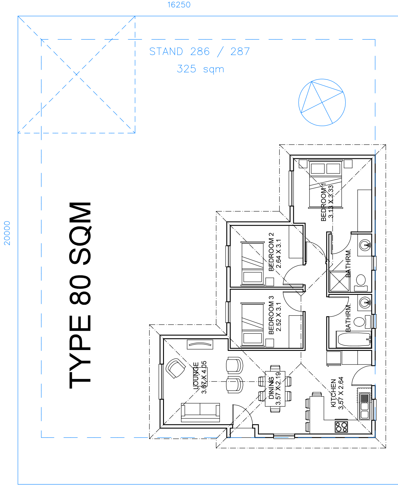
GROUND FLOOR PLAN 80.01 m 2
