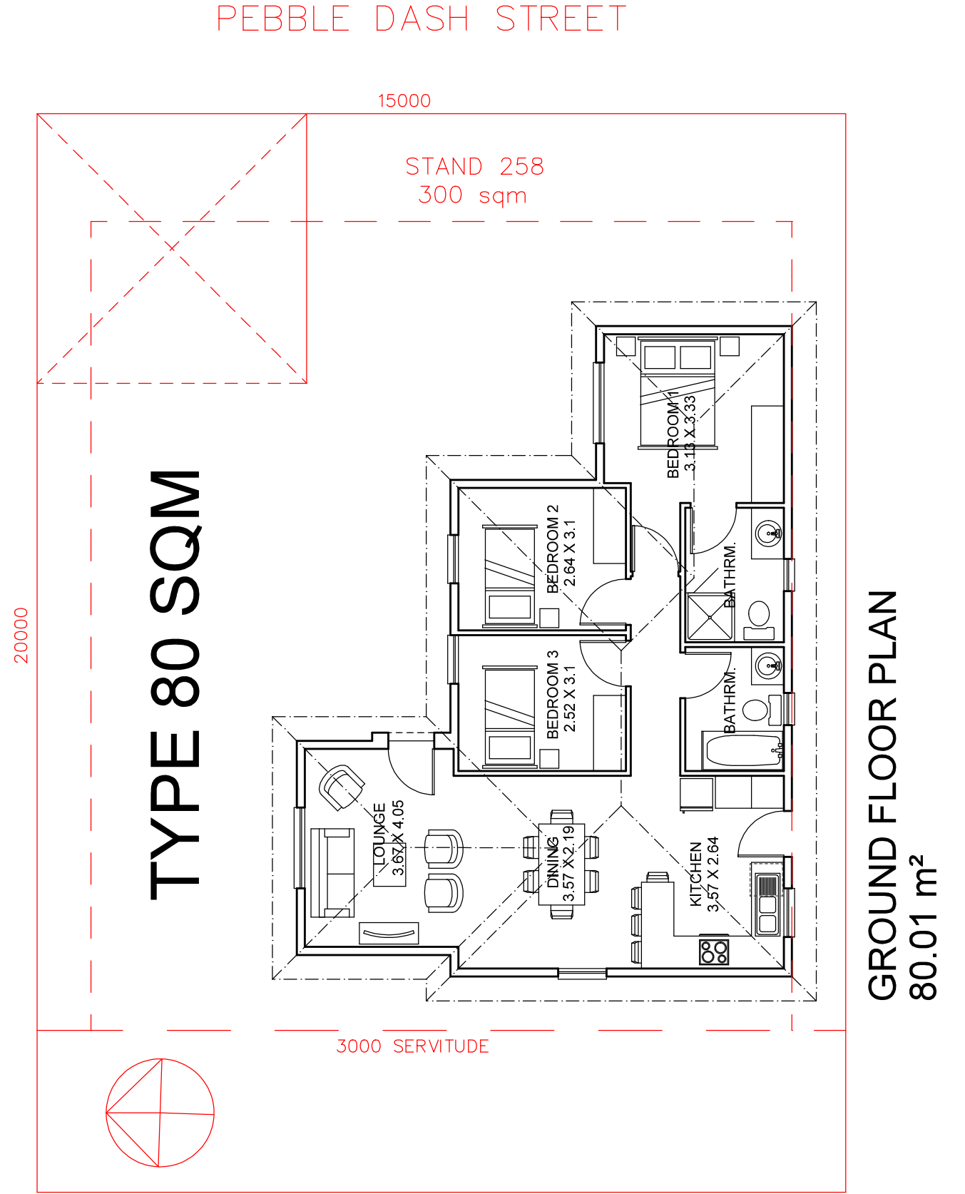
GROUND FLOOR PLAN 80.01 m 2
