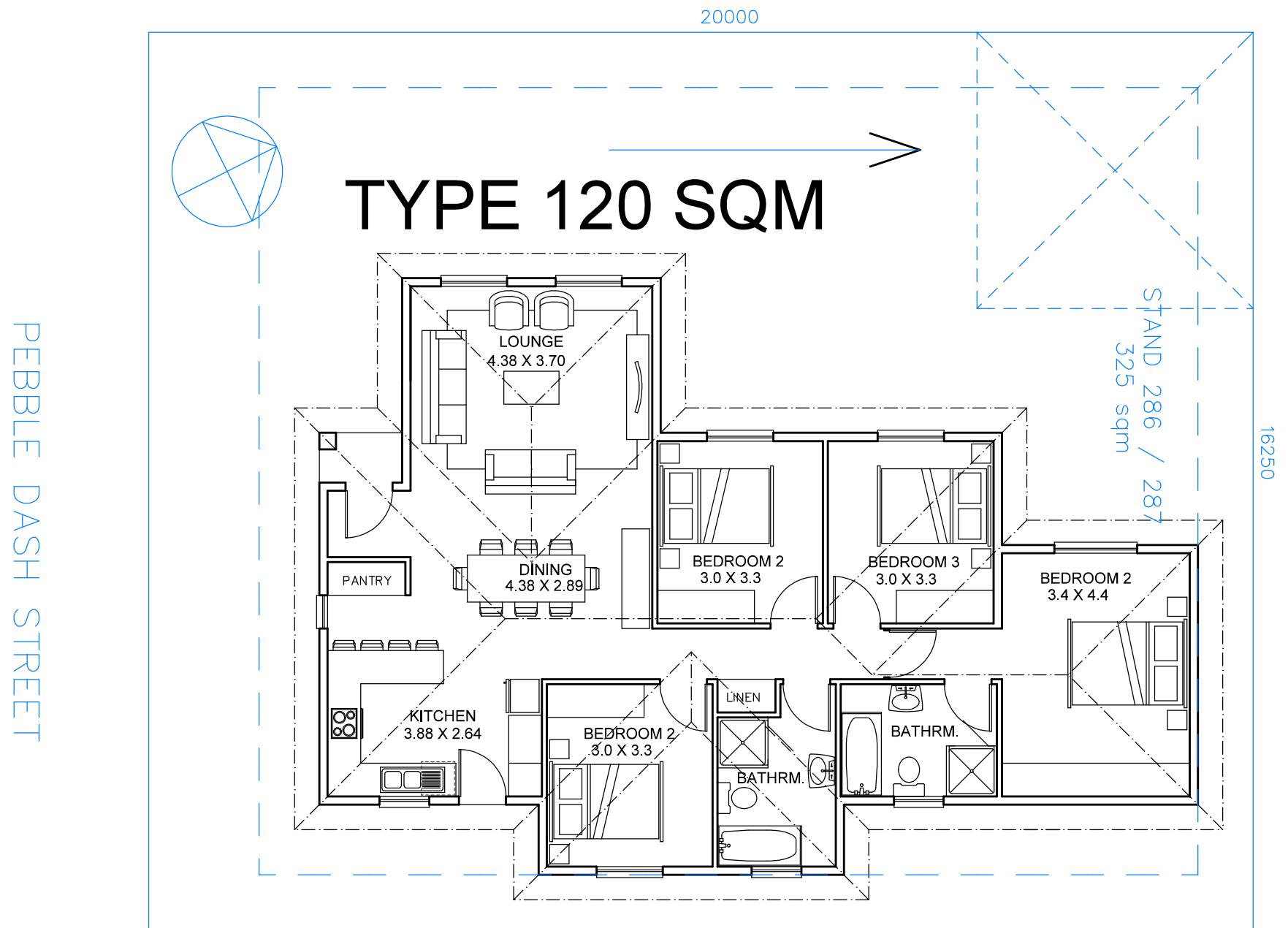
GROUND FLOOR PLAN 120.00 m 2
