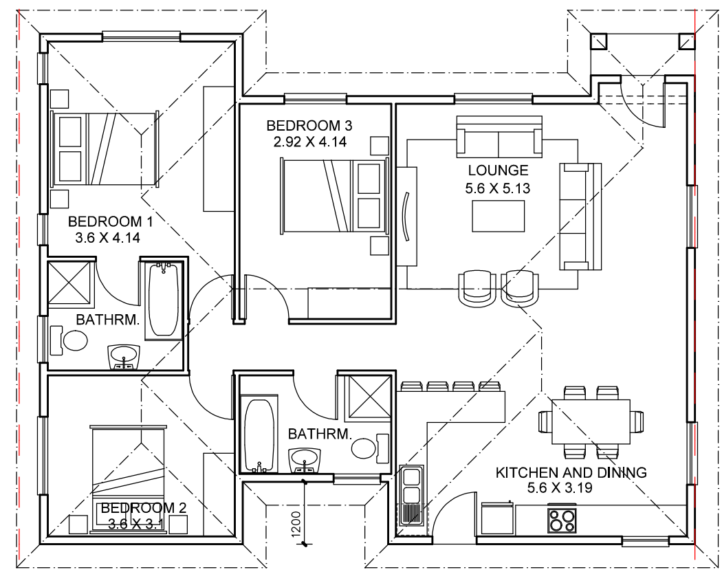
GROUND FLOOR PLAN 112.33 m 2
