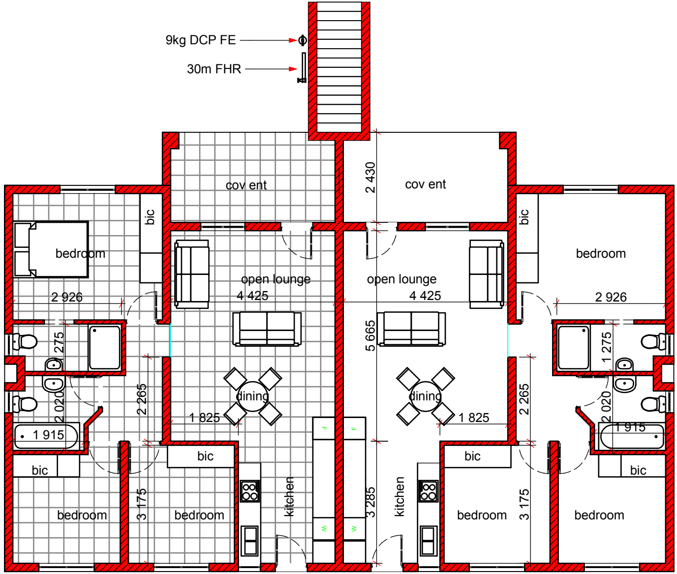
GROUND STOREY PLAN
