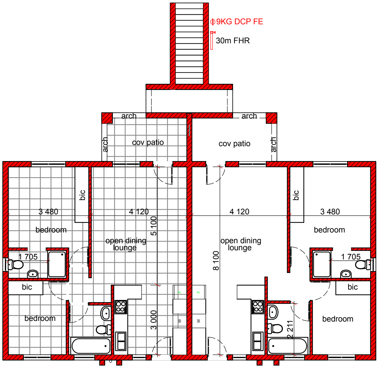
GROUND STOREY PLAN 2 BED RM 1:100
